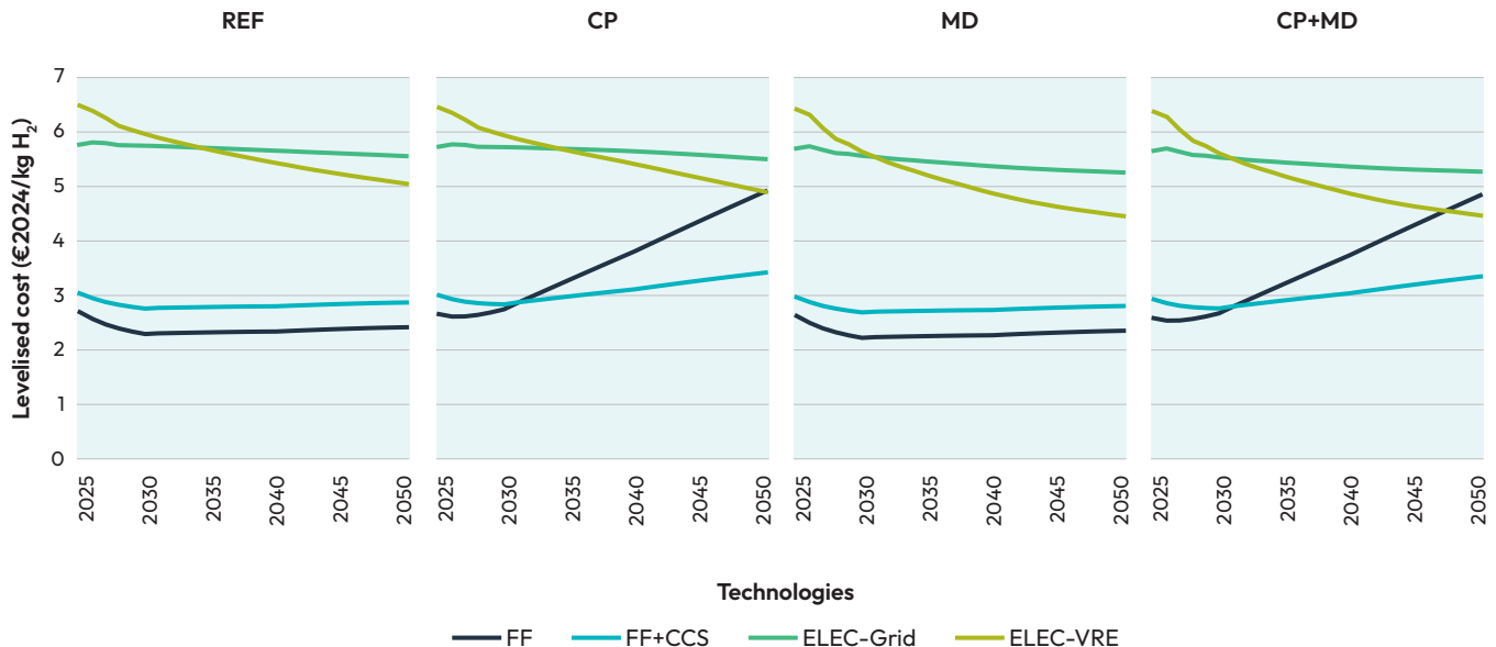
Figure 3: Global average levelised cost of hydrogen production by each technology group in each policy scenario. Global averages are unweighted and regional estimates vary a lot.
