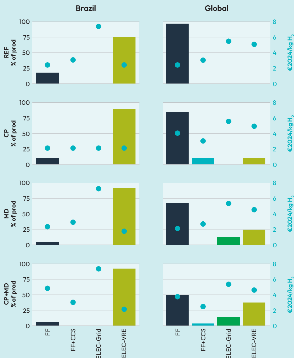
Figure 7: Comparison of hydrogen production in Brazil versus the world in each scenario for 2050.
