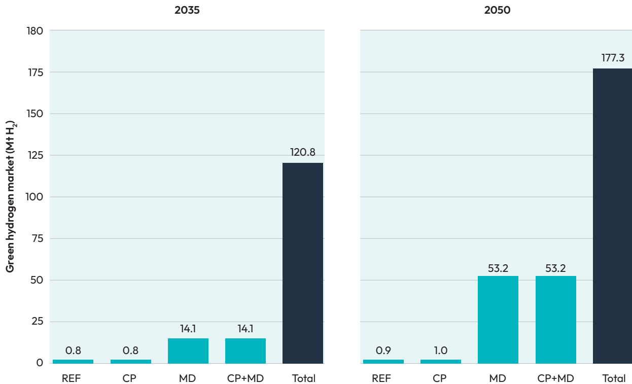
Figure 6: Global electrolytic hydrogen demand (shown in blue) in the various scenarios relative to total hydrogen demand (shown in black)
