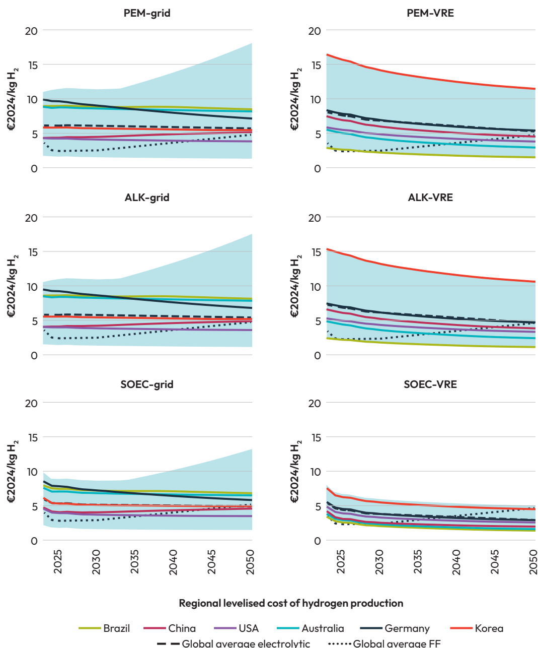
Figure 5: Levelised cost of electrolytic hydrogen production under the CP+MD scenario by selected model region 19
